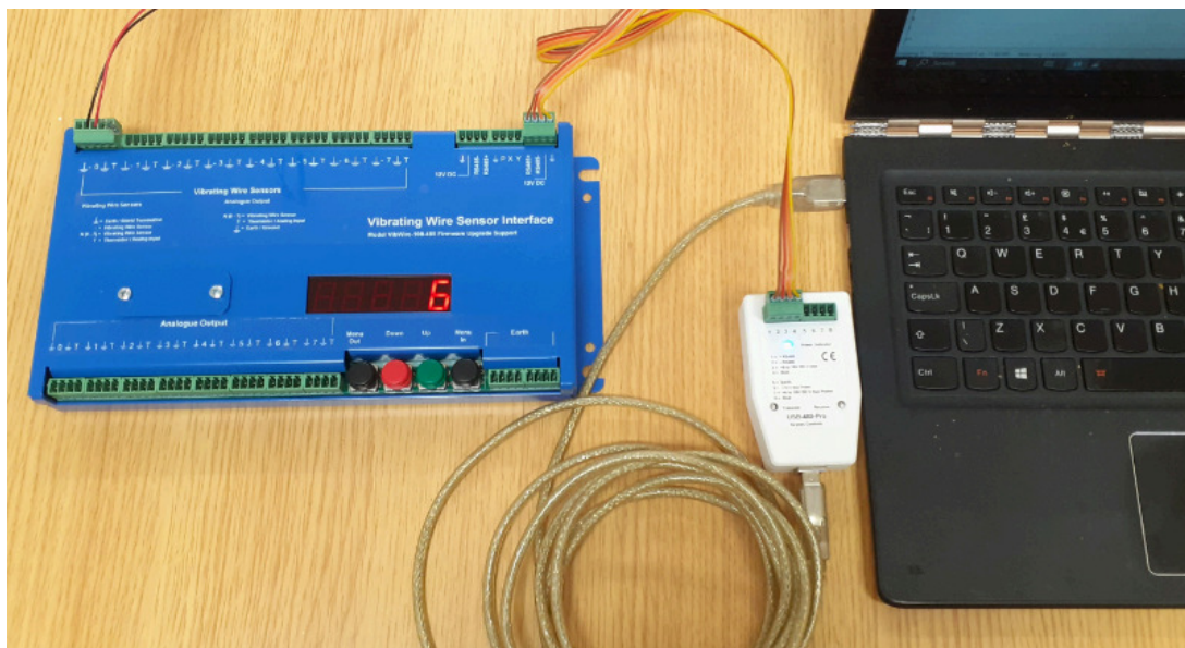
Figure 13 - Media Converter connection to the VibWire-108
