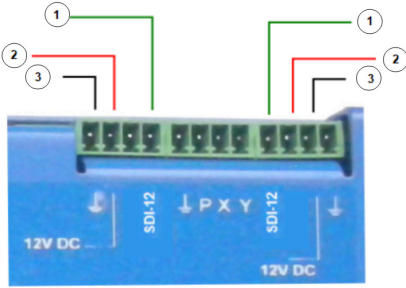
SDI-12 Network Connection
