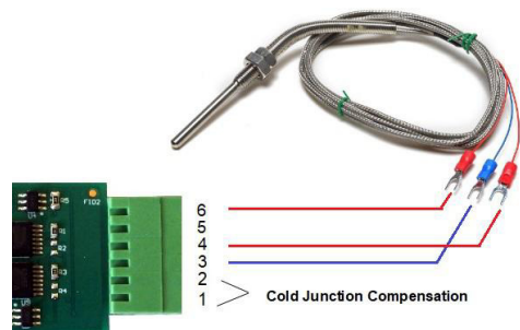
Figure 7 - IEC 60751-2008 PT500 RTD Sensor
