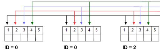
Multiple Device RS485 Network Connection - Figure 6
