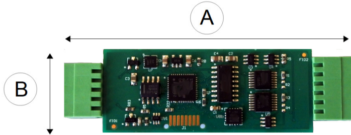
Dimensions A = Length 75 mm B = 24 mm
